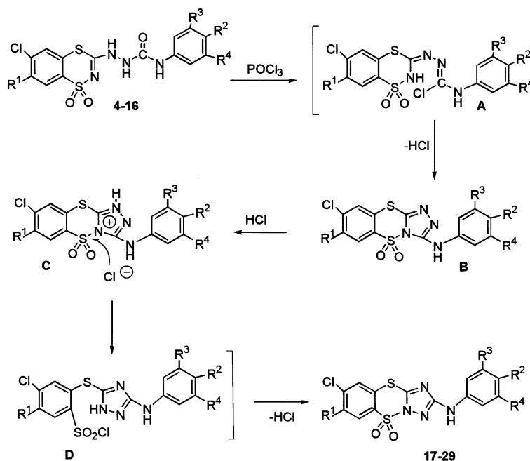
Scheme 2. Proposed mechanism of the formation of the 2-arylmino-5,5-dioxo[1,24]triazolo[2,3- b ][1,4,2]benzodithiazines 17–29 .
